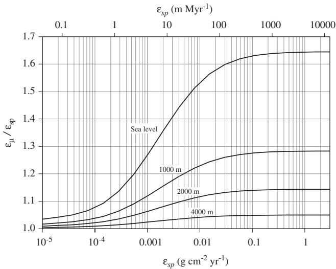
Fig. 8. Difference between calculated erosion rates from a high-latitude sample that take account of subsurface nuclide production by muons ( \epsilon_{\mu} ; Eq. (2)) and those that do not ( \epsilon_{sp} ; Eq. (3)). The two different x-axis scales are related by a density of 2.65 \text{ g cm}^{-3} .
