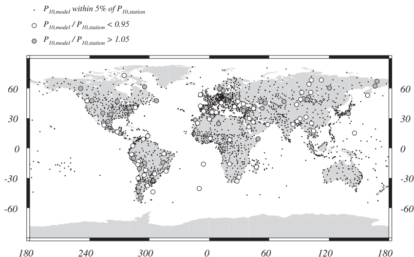
Fig. 2. Geographic representation of the accuracy of the atmospheric pressure–elevation relationship used in the online calculator. The points on the map are the locations of meteorological stations in the NCAR World Monthly Surface Station Climatology data set (see text for details). The same data are shown in Fig. 1. The small dots show stations where the ^{10}\text{Be} production rate estimated from the location of the station and our default atmospheric pressure–elevation relationship (that draws sea level pressure and 1000 mbar temperature from the NCEP reanalysis, as described in the text) is within 5% of the ^{10}\text{Be} production rate estimated from the mean atmospheric pressure actually recorded at the station. White circles show stations where the production rate calculated using our pressure–elevation relationship is more than 5% lower than the production rate calculated from the actual station pressure; gray circles show stations where it is more than 5% higher. Stations south of 60^\circ\text{S} are not included. As discussed in the caption for Fig. 1, we did not make a comprehensive effort to screen the data set for errors. Thus, this figure is intended only as a general guideline to identify regions where the default pressure–elevation relationship in the calculators may result in inaccurate exposure ages.
